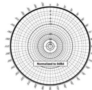
Azimuthal Pattern (Y, Z, or E-plane)
